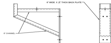
STEEL BUMPER
